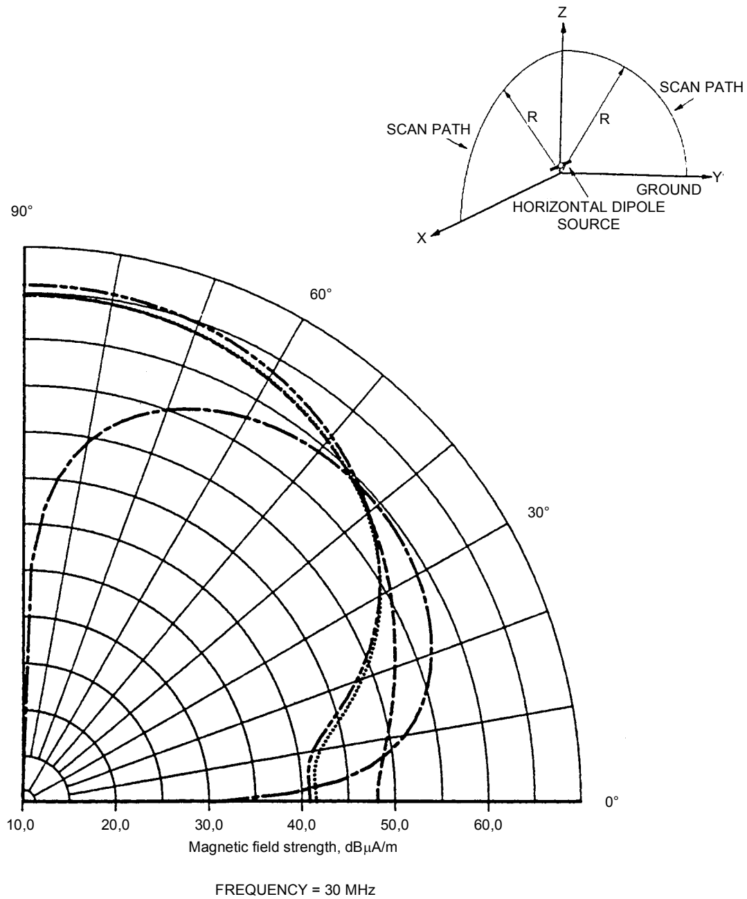
Figure 4.6-55 – Vertical radiation patterns of the H -fields emitted by a small horizontal electric dipole located close to the ground
