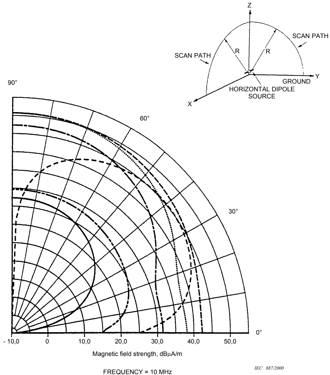
Figure 4.6-46 – Vertical radiation patterns of the H -fields emitted by a small horizontal electric dipole located close to the ground
