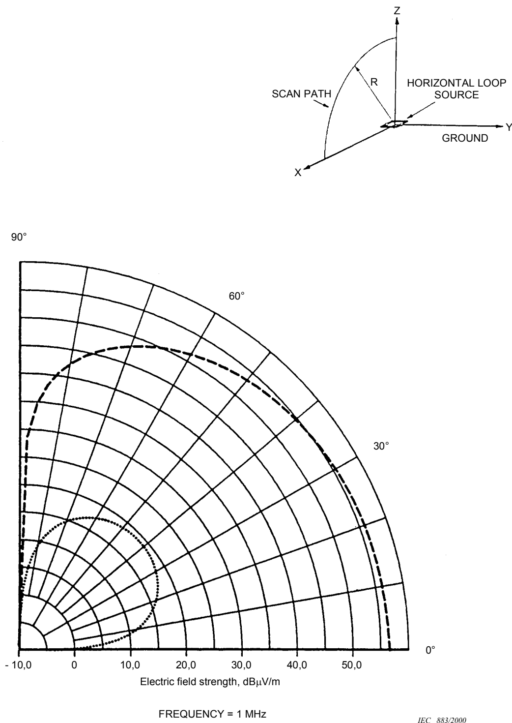
Figure 4.6-42 – Vertical radiation patterns of the E -fields emitted by a small vertical magnetic dipole (horizontal loop) located close to the ground
