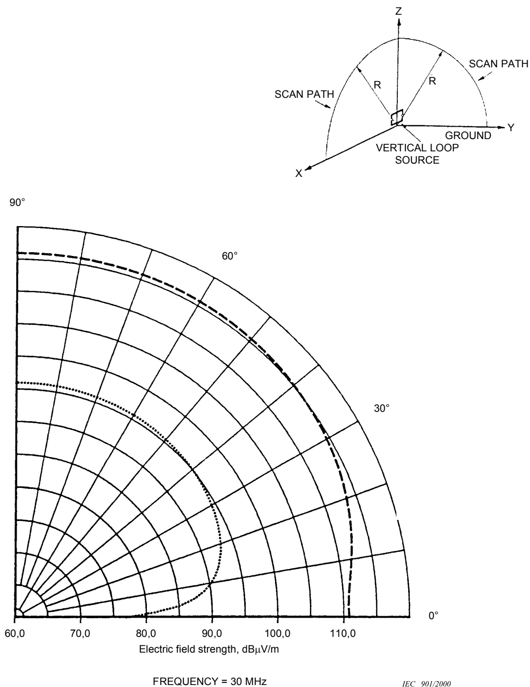
Figure 4.6-60 – Vertical radiation patterns of the vertically polarized E -fields emitted by a small horizontal magnetic dipole (vertical loop) located close to the ground
