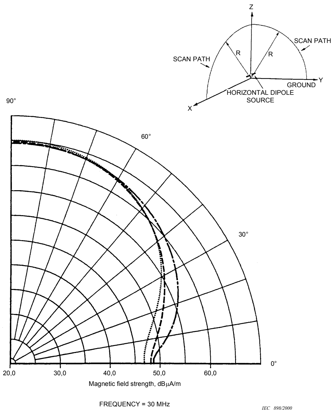
Figure 4.6-57 – Influence of a wide range of values of the electrical constants of the ground on the vertical radiation patterns of the horizontally oriented H -fields emitted by a small horizontal electric dipole located close to the ground
