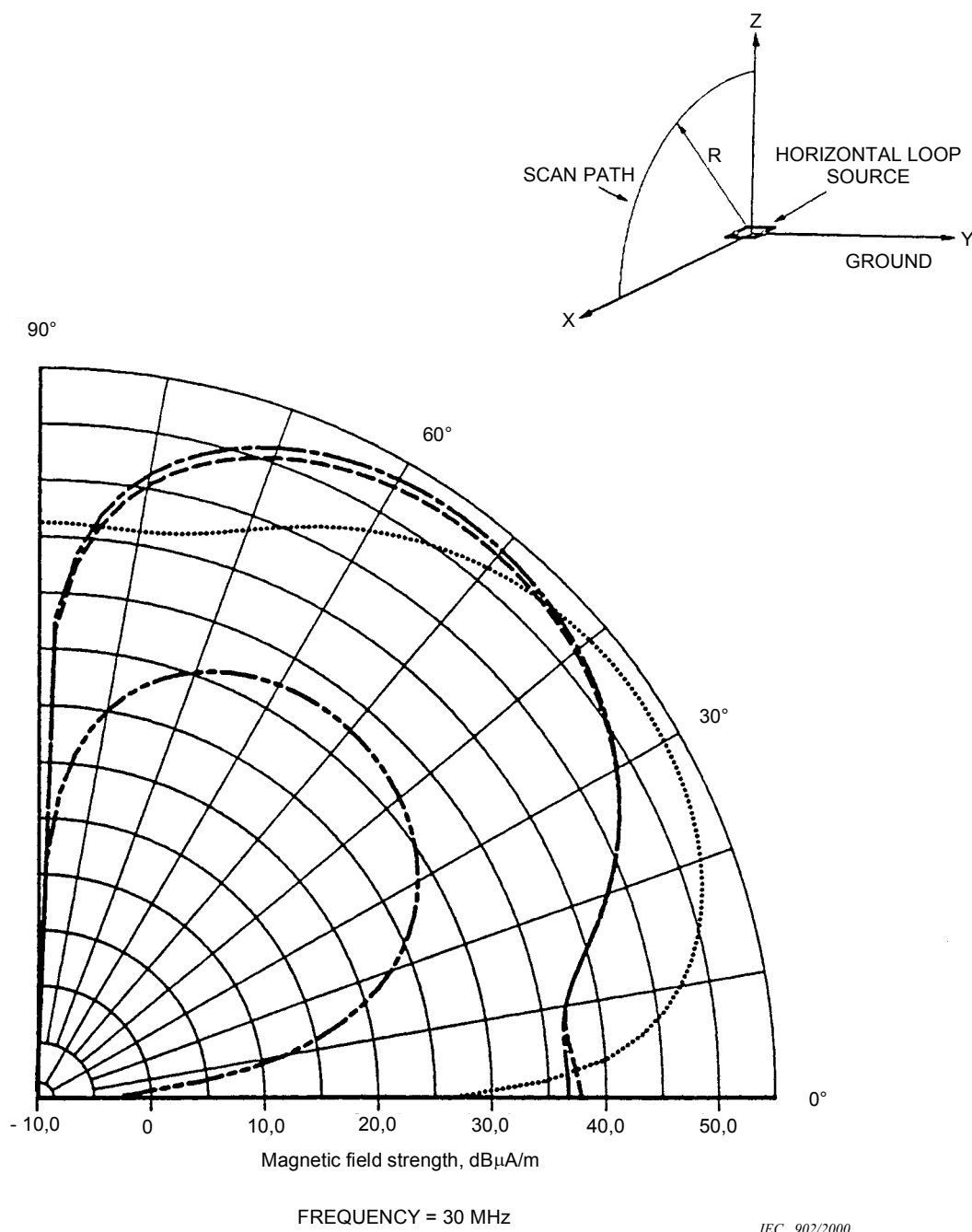
Figure 4.6-61 – Vertical radiation patterns of the H -fields emitted by a small vertical magnetic dipole (horizontal loop) located close to the ground
