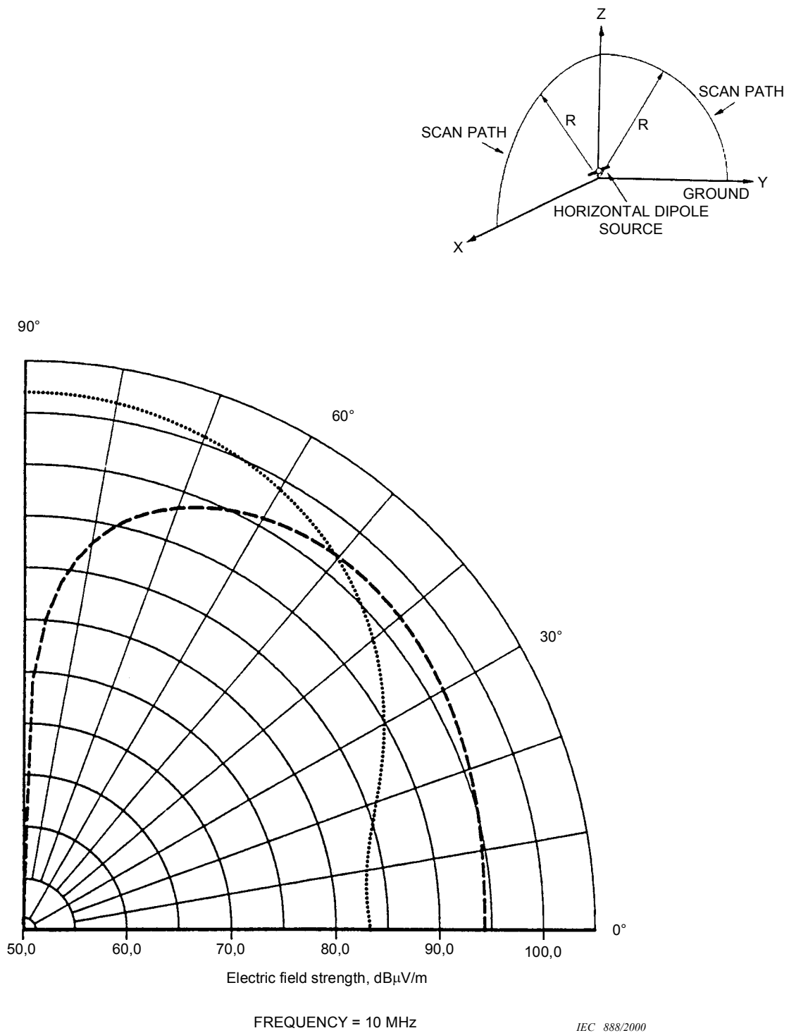
Figure 4.6-47 – Vertical radiation patterns of the E -fields emitted by a small horizontal electric dipole located close to the ground
