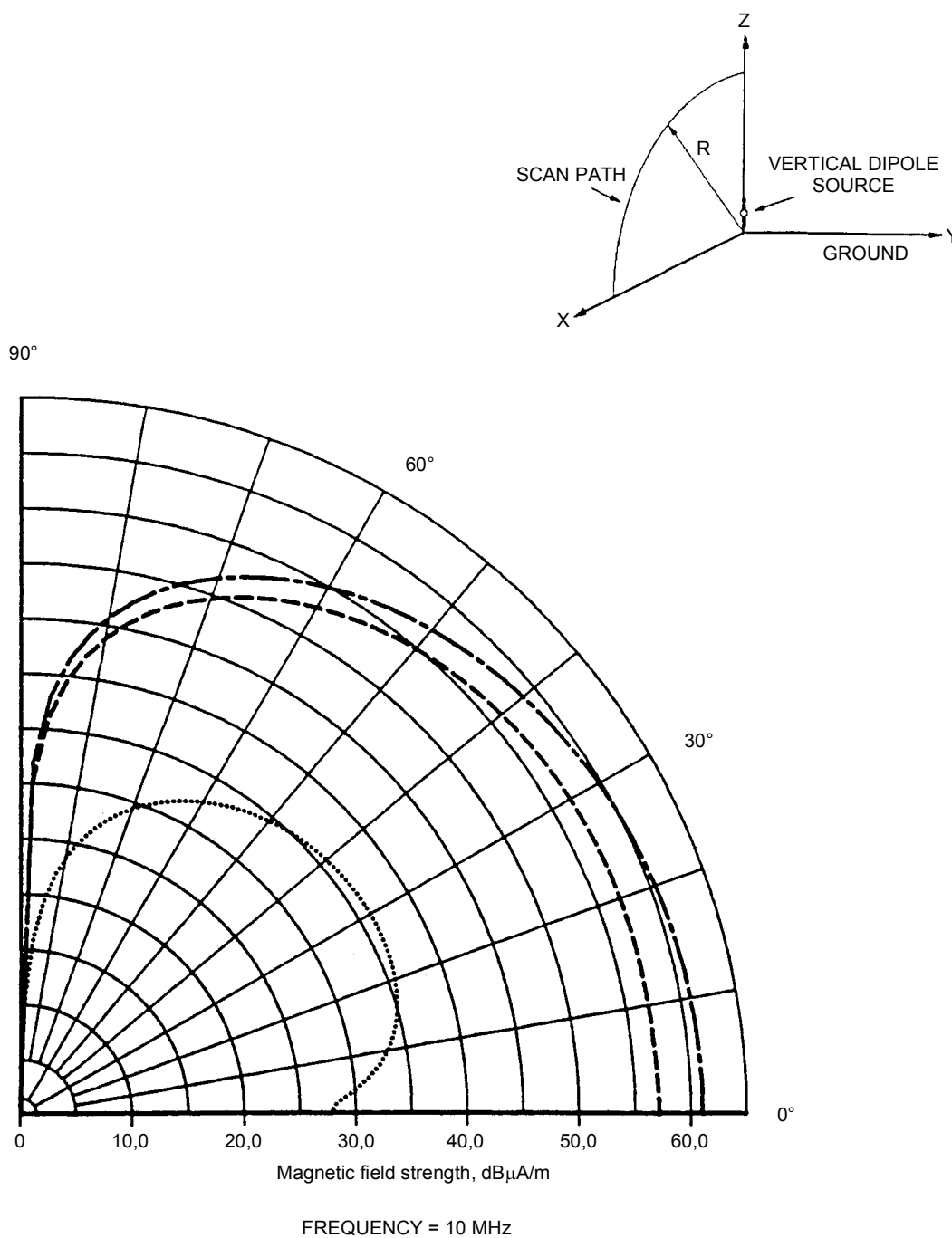
Figure 4.6-43 – Vertical radiation patterns of the horizontally oriented H -fields emitted by a small vertical electric dipole located close to the ground
