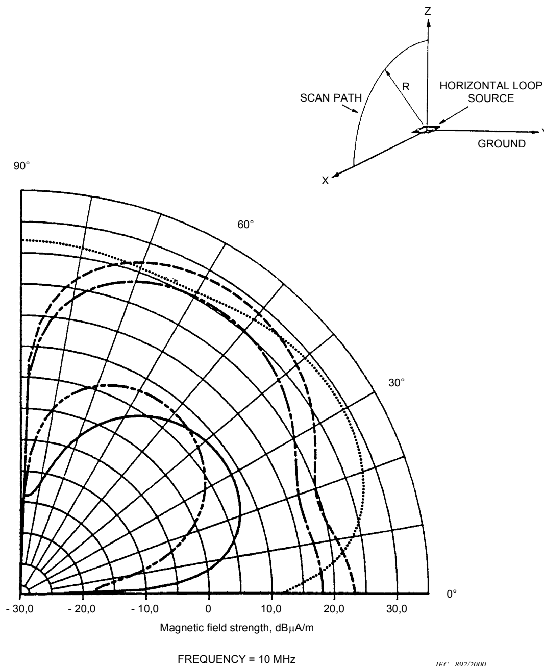
Figure 4.6-51 – Vertical radiation patterns of the H -field emitted by a small vertical magnetic dipole (horizontal loop) located close to the ground
