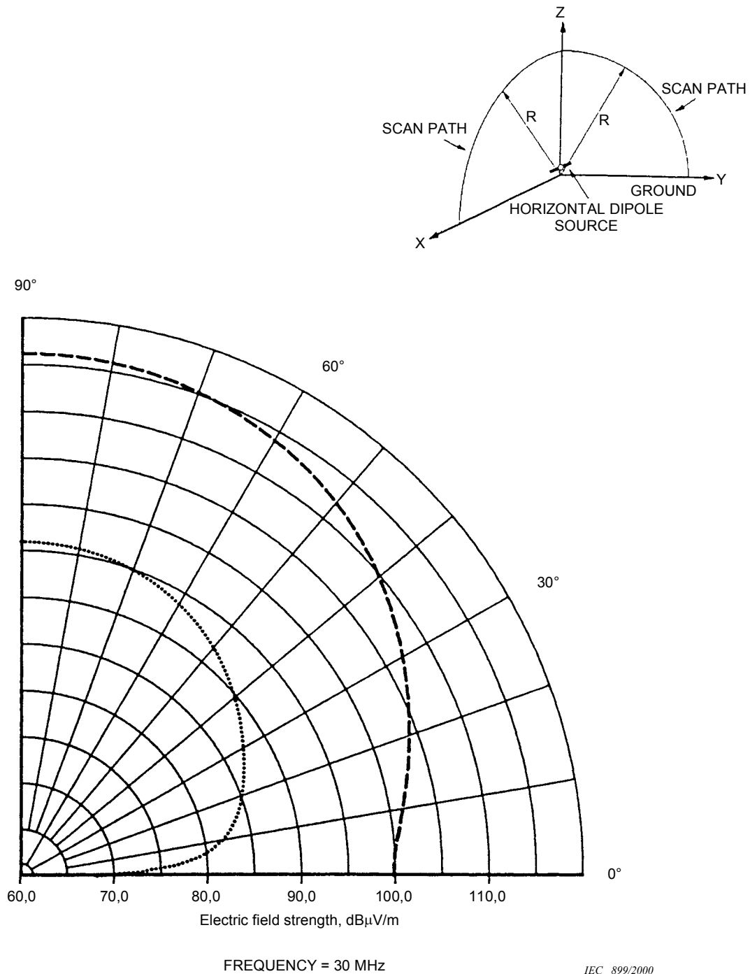
Figure 4.6-58 – Vertical radiation patterns of the vertically polarized E -fields emitted by a small horizontal electric dipole located close to the ground
