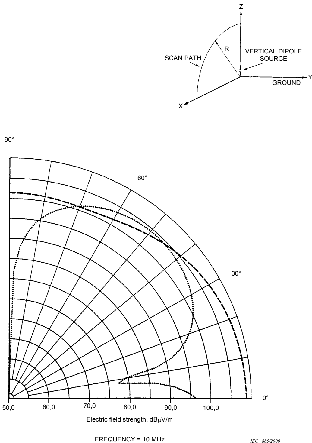
Figure 4.6-44 – Vertical radiation patterns of the E -fields emitted by a small vertical electric dipole located close to the ground
