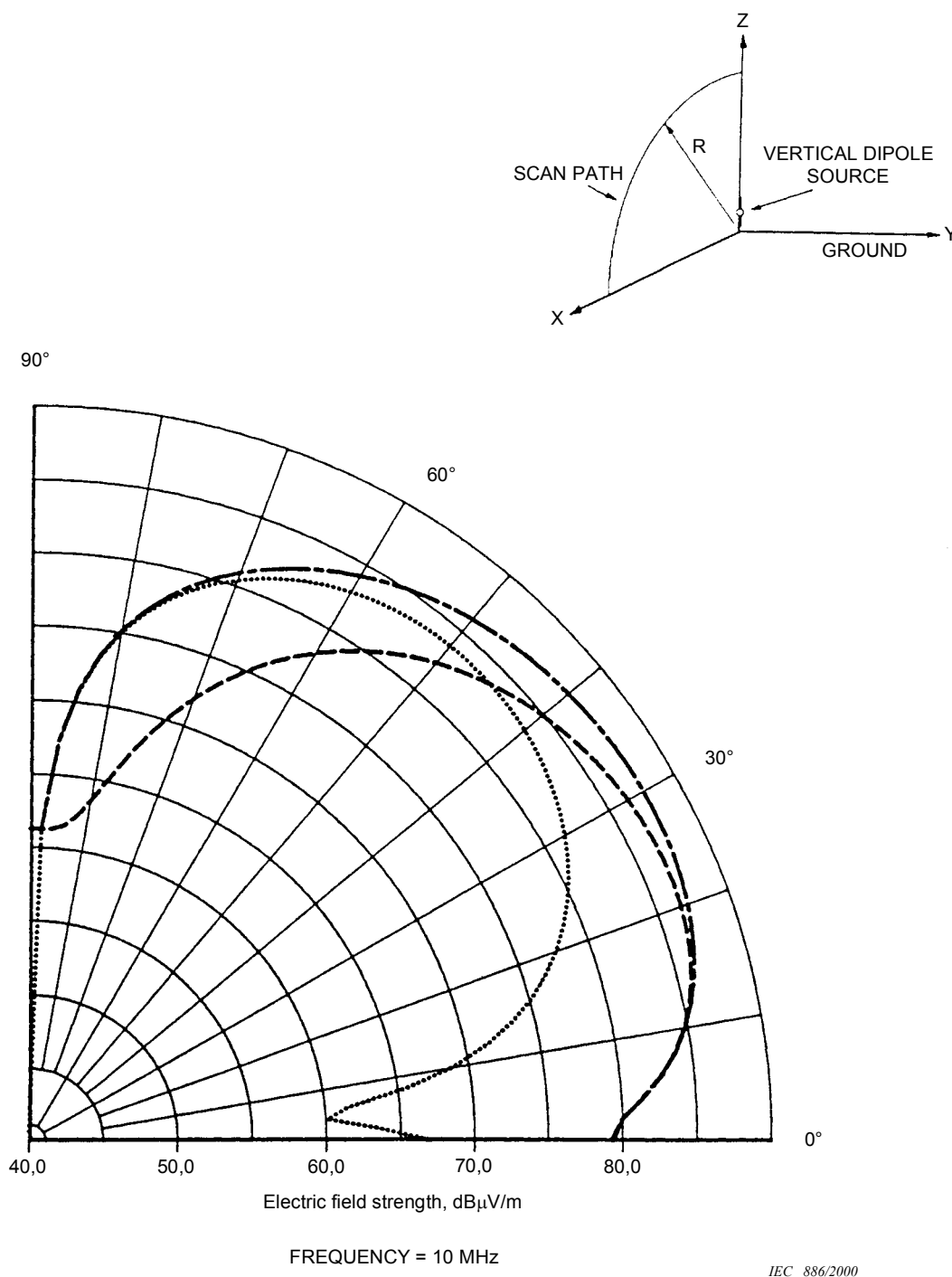
Figure 4.6-45 – Vertical radiation patterns of the E -fields emitted by a small vertical electric dipole located close to the ground
