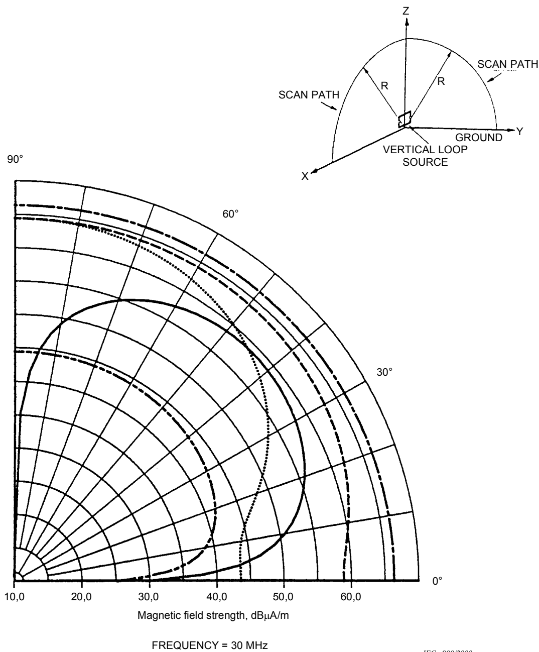
Figure 4.6-59 – Vertical radiation patterns of the H -fields emitted by a small horizontal magnetic dipole (vertical loop) located close to the ground
