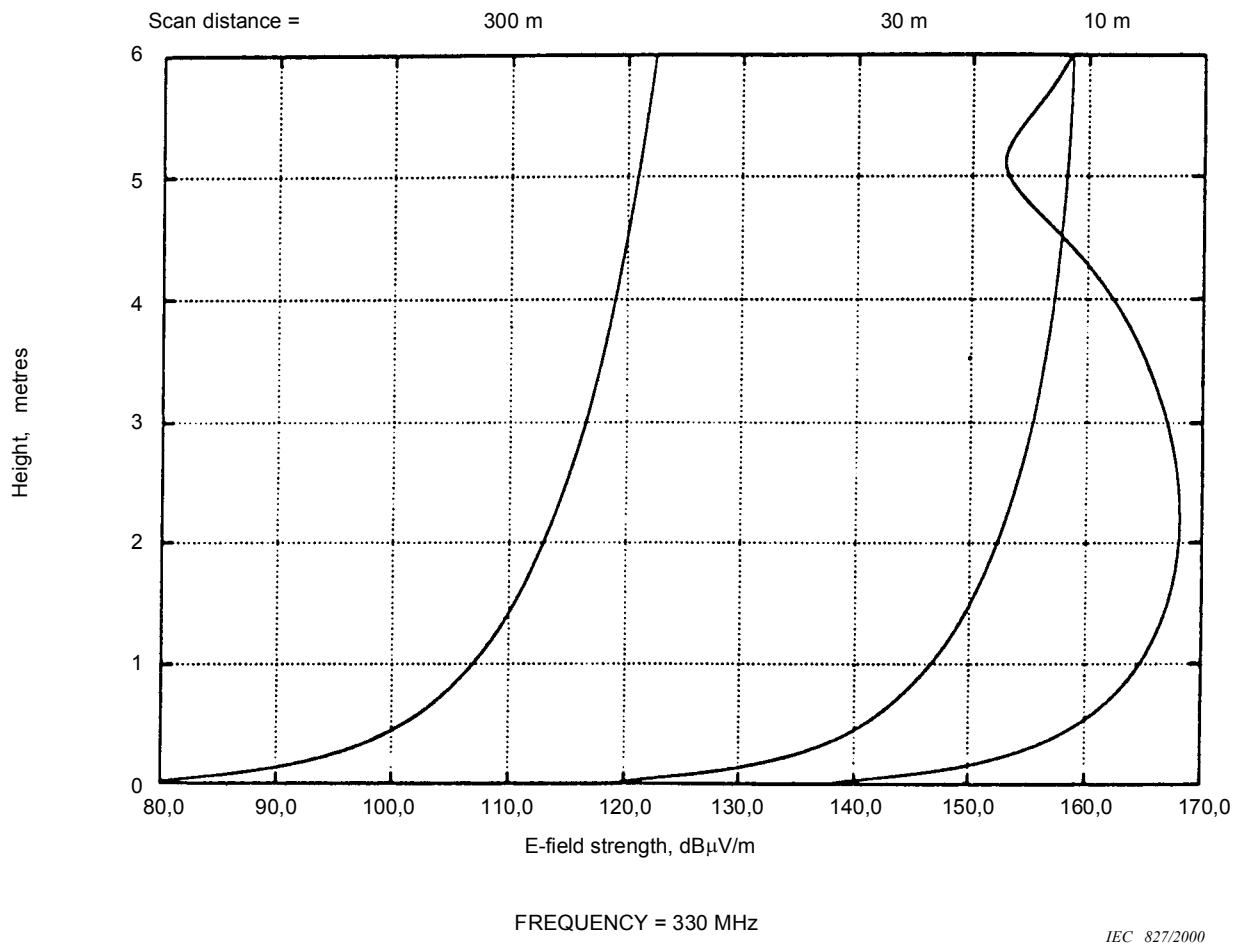
Figure 4.5-11(b) – Height scan patterns of horizontally polarized E -field strength emitted at 330 MHz from the small horizontal loop (vertical magnetic dipole), at horizontal distances of 10 m, 30 m and 300 m in the Z-X plane. Loop dimensions 0,05 m \times 0,05 m. Loop height 1 m. Dipole moment 1 A·m 2 . Ground constants: \epsilon_r = 15 , \sigma = 4,5 mS/m. (Reproduced from [10])
