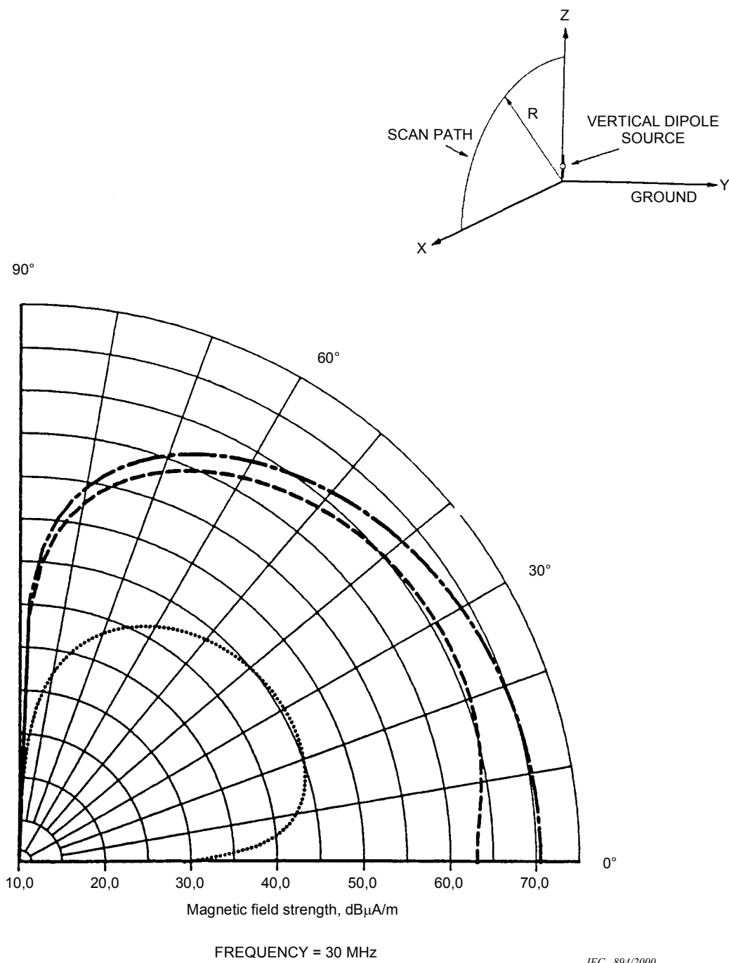
Figure 4.6-53 – Vertical radiation patterns of the horizontally oriented H -fields emitted by a small vertical electric dipole located close to the ground
