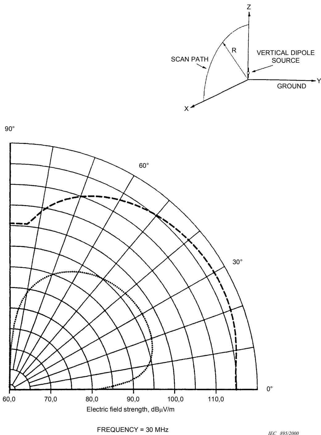
Figure 4.6-54 – Vertical radiation patterns of the vertically polarized E -fields emitted by a small vertical electric dipole located close to the ground
