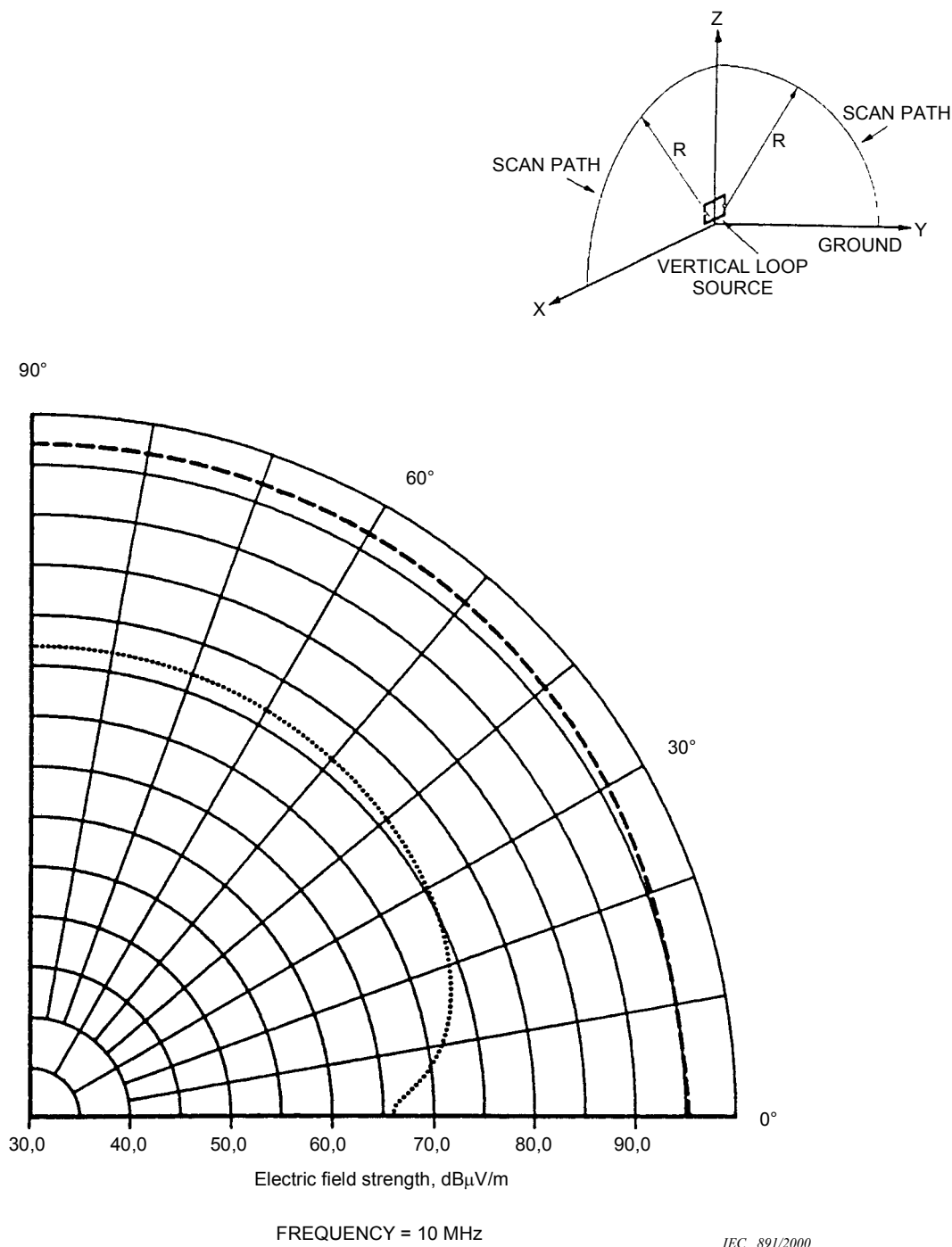
Figure 4.6-50 – Vertical radiation patterns of the vertically polarized E -fields emitted by a small horizontal magnetic dipole (vertical loop) located close to the ground
