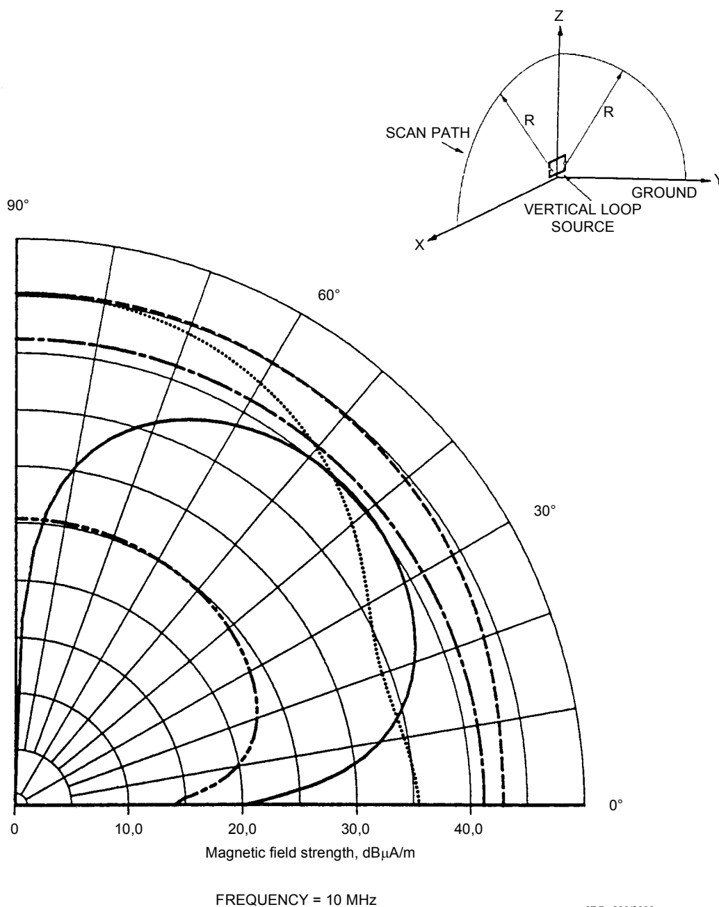
Figure 4.6-49 – Vertical radiation patterns of the H -field emitted by a small horizontal magnetic dipole (vertical loop) located close to the ground
