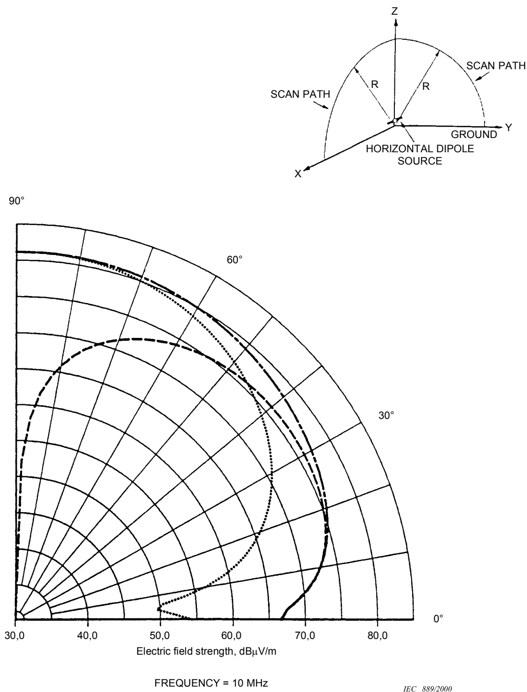
Figure 4.6-48 – Vertical radiation patterns of the E -fields emitted by a small horizontal electric dipole located close to the ground
