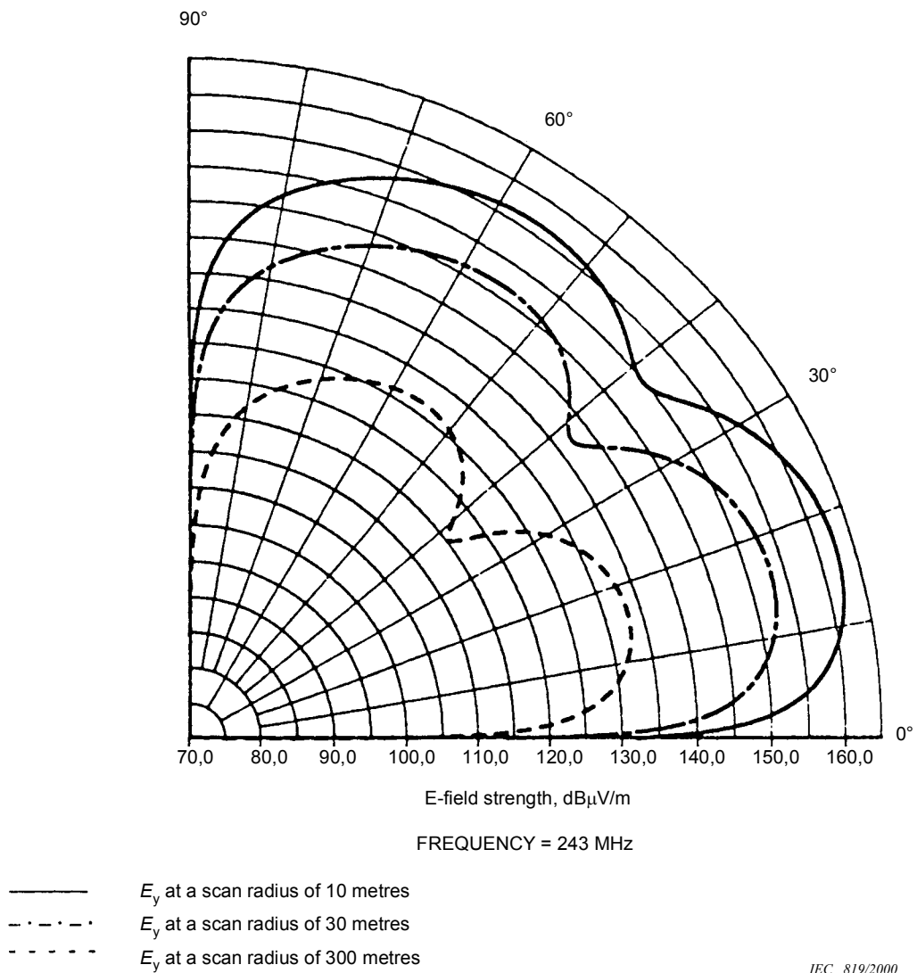
Figure 4.5-8(a) – Vertical polar patterns of horizontally polarized E -field strength emitted at 243 MHz around the small horizontal loop (vertical magnetic dipole), at scan radii of 10 m, 30 and 300 m in the Z-X plane. Loop dimensions 0,05 m \times 0,05 m. Loop height 1 m. Dipole moment 1 A·m 2 . Ground constants: \epsilon_r = 15 , \sigma = 4,5 mS/m. (Reproduced from [10])
