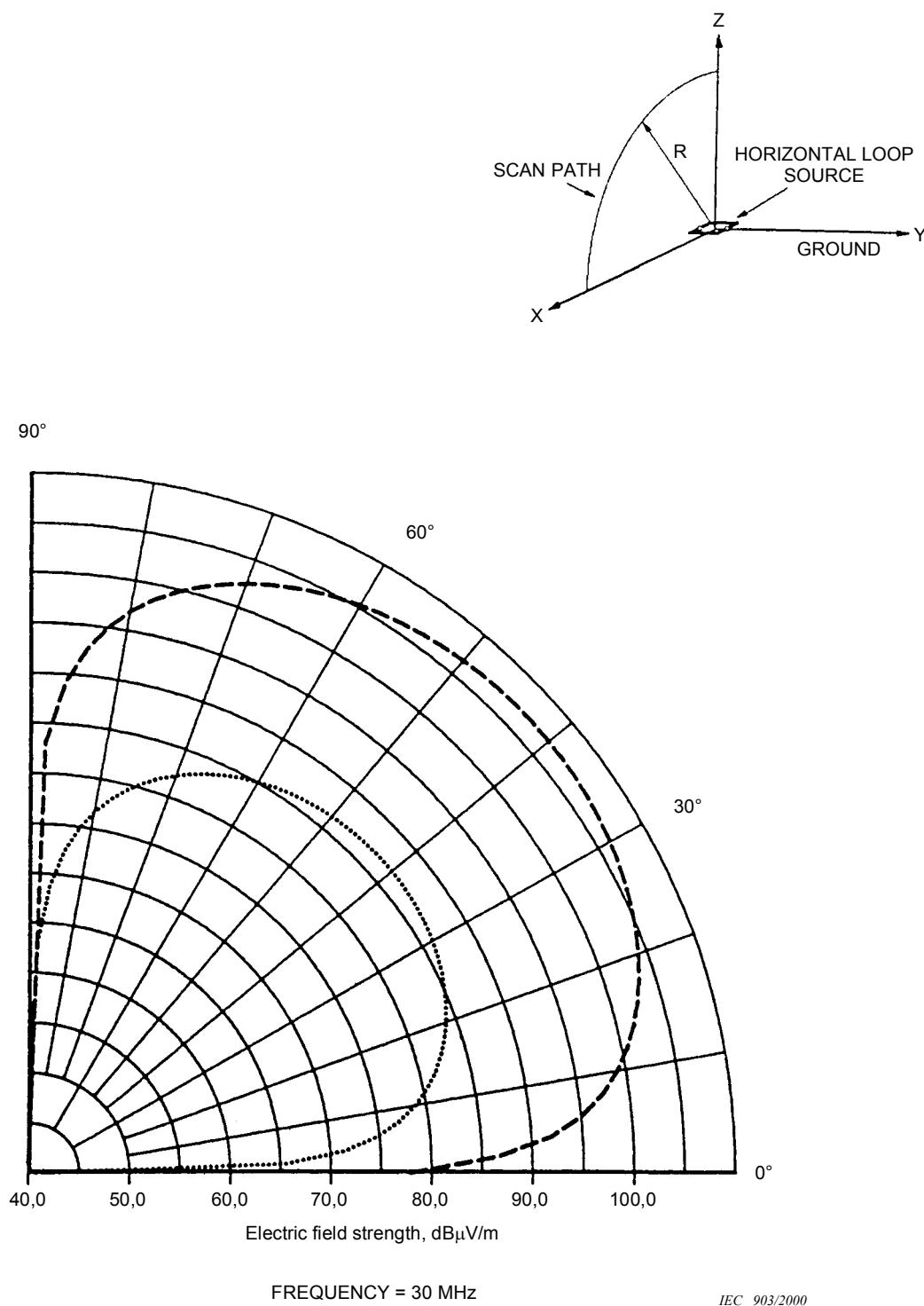
Figure 4.6-62 – Vertical radiation patterns of the E -fields emitted by a small vertical magnetic dipole (horizontal loop) located close to the ground
