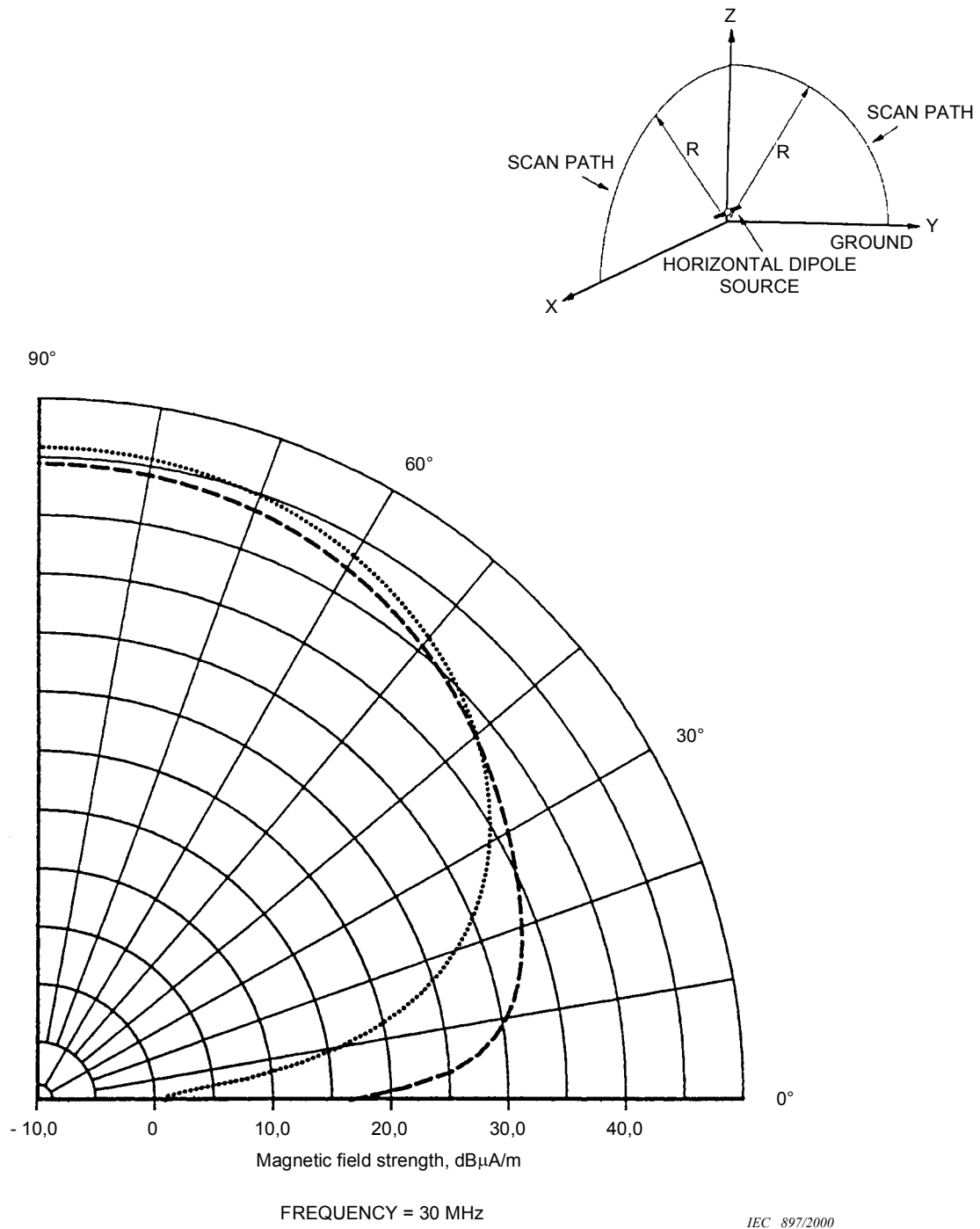
Figure 4.6-56 – Vertical radiation patterns of the horizontally oriented H -fields emitted by a small horizontal electric dipole located close to the ground
