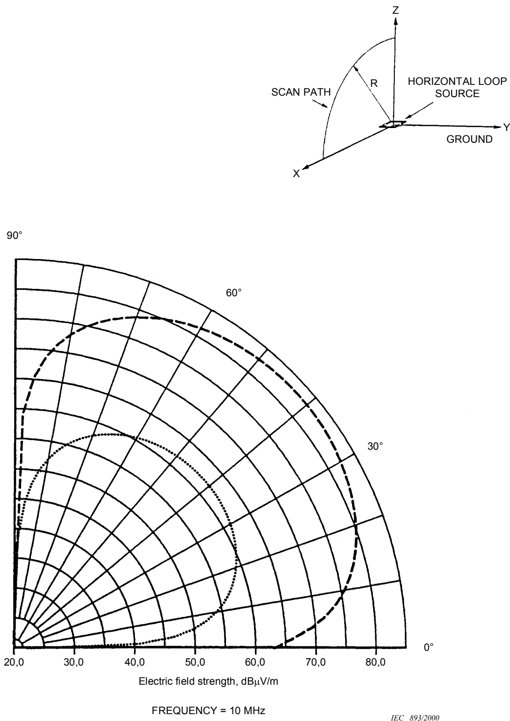
Figure 4.6-52 – Vertical radiation patterns of the E -fields emitted by a small vertical magnetic dipole (horizontal loop) located close to the ground
